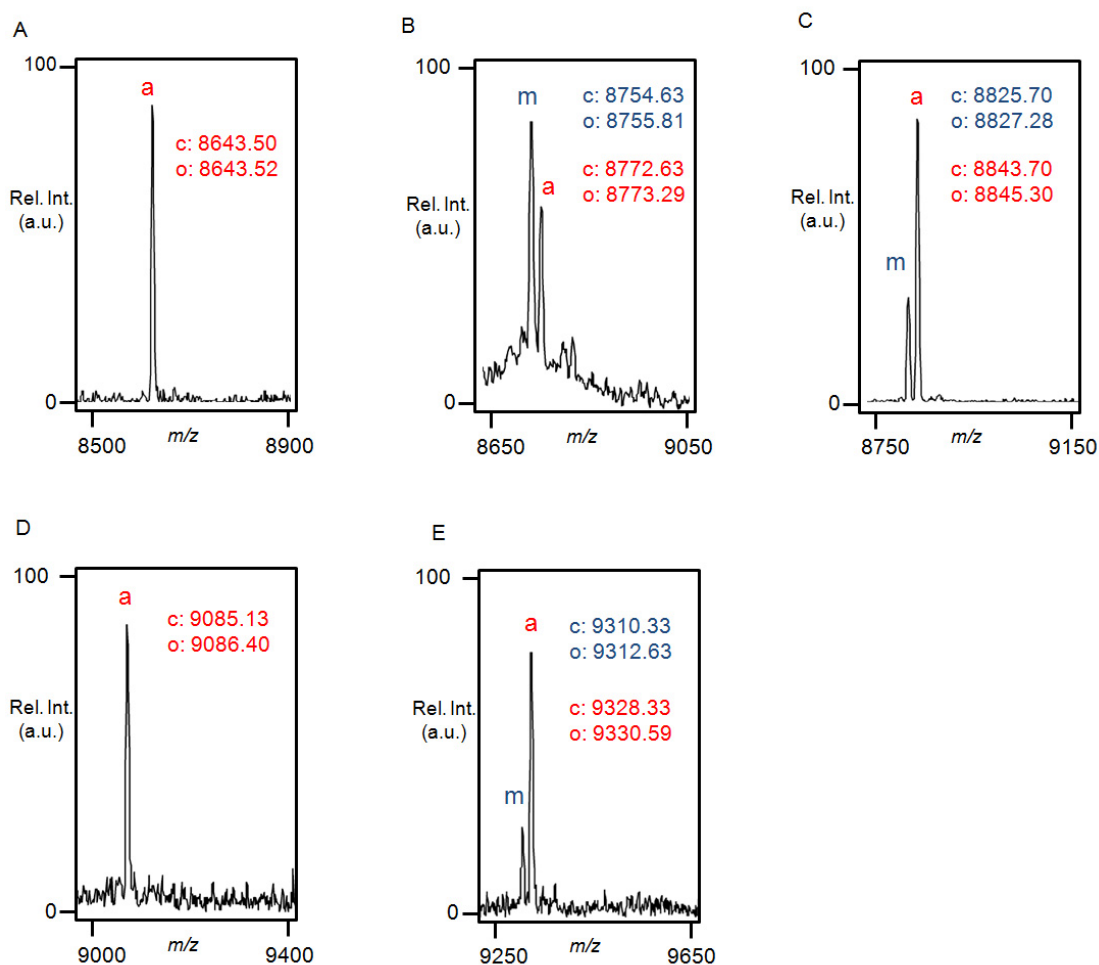
Supplementary Figure S6. MALDI-TOF spectra of the products obtained from the MeaF-containing constructs as isolated from E. coli cells after 12-hour expression using pH 8.0 buffer containing iodoacetamide. (A) CBD-6T(MeaF); (B) CBD-7T(MeaF); (C) CBD-8T(MeaF); (D) CBD-10T(MeaF); and (E) CBD-12T(MeaF). "m" = macrolactam (S-carboxyamidomethyl adduct), "a" = acyclic side product (S-carboxyamidomethyl adduct). The calculated ("c") and observed ("o") m/z values corresponding to the [M+H]^+ adducts are indicated and color coded.
