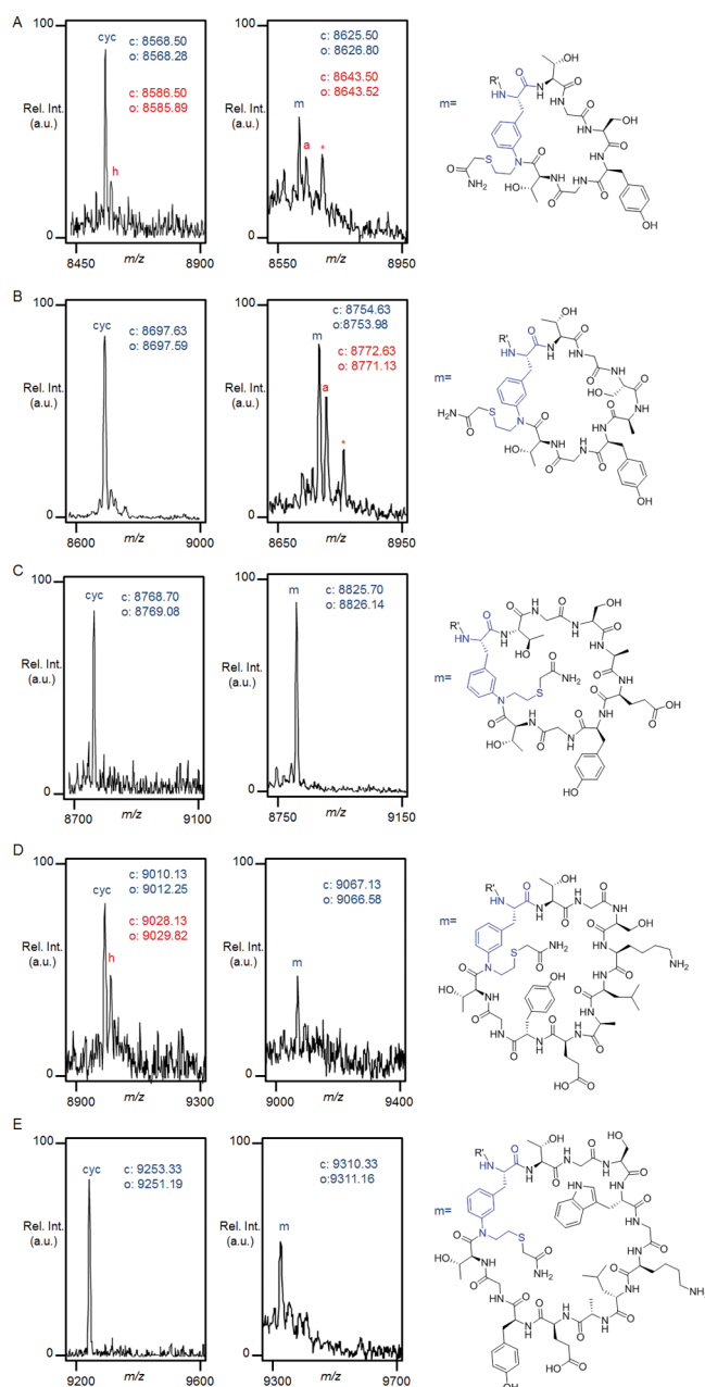
Figure 6. MALDI-TOF spectra of the macrocyclization products obtained from the MeaF-containing constructs as isolated from E. coli cells after 12 h (left panel) and 24 h (right panel) using pH 5.0 and 8.0 buffers containing iodoacetamide, respectively. (A) CBD-6T(MeaF); (B) CBD-7T(MeaF); (C) CBD-8T(MeaF); (D) CBD-10T(MeaF); and (E) CBD-12T(MeaF). See also Figures S5 and S6. cyc, macrocyclic product in either thiolactone or lactam form; h, hydrolyzed product; m, macrolactam (S-carboxyamidomethyl adduct); a, acyclic side product (S-carboxyamidomethyl adduct); *, acetylated a. The calculated (c) and observed (o) m/z values corresponding to the [M + H]^+ adducts are indicated and color-coded.
