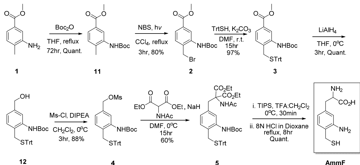
Scheme S1: Synthesis of AmmF
