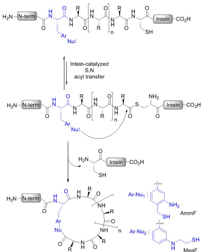
Figure 1. Overview of the strategy for generating side chain-to-tail macrocyclic peptides via cyclization of ribosomally derived, intein-fused precursor proteins by means of aminothiol unnatural amino acids. Nu refers to the nucleophilic 1,3- or 1,2-aminothiol moiety.
