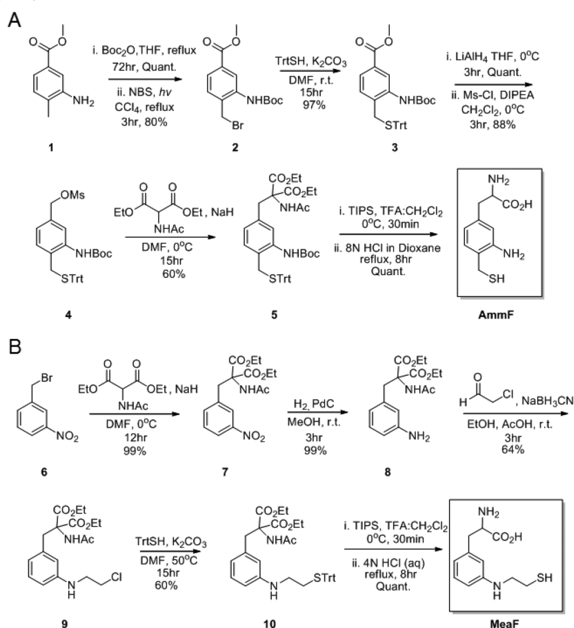
Scheme 1. Synthetic Routes for the Preparation of (A) 3-Amino-4-mercaptomethyl-phenylalanine (AmmF) and (B) 3-(2-Mercapto-ethyl)amino-phenylalanine (MeaF)
