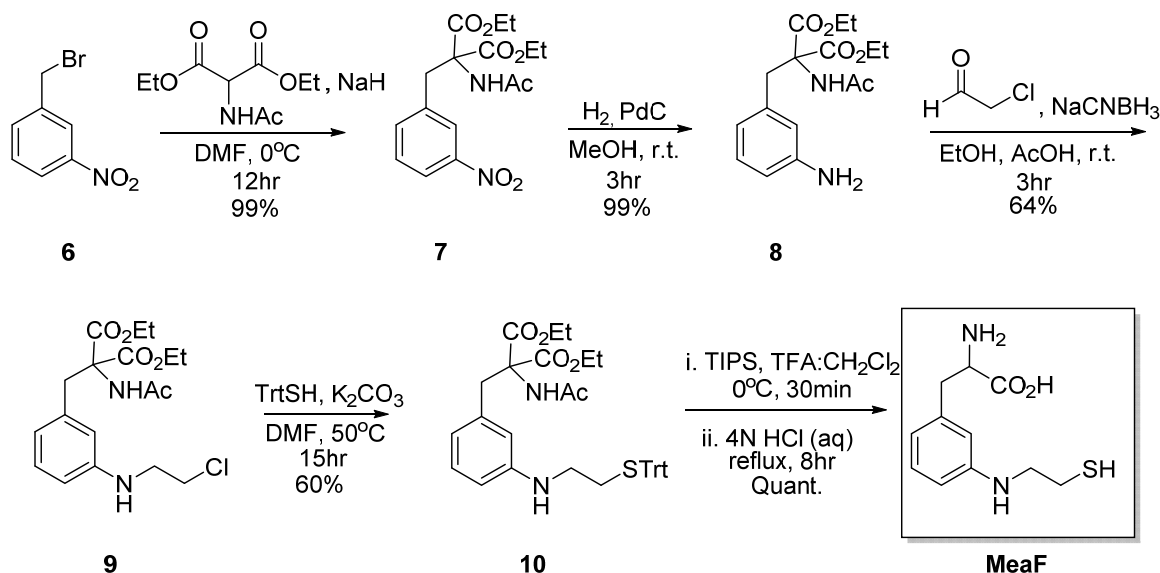
Scheme S2: Synthesis of MeaF
