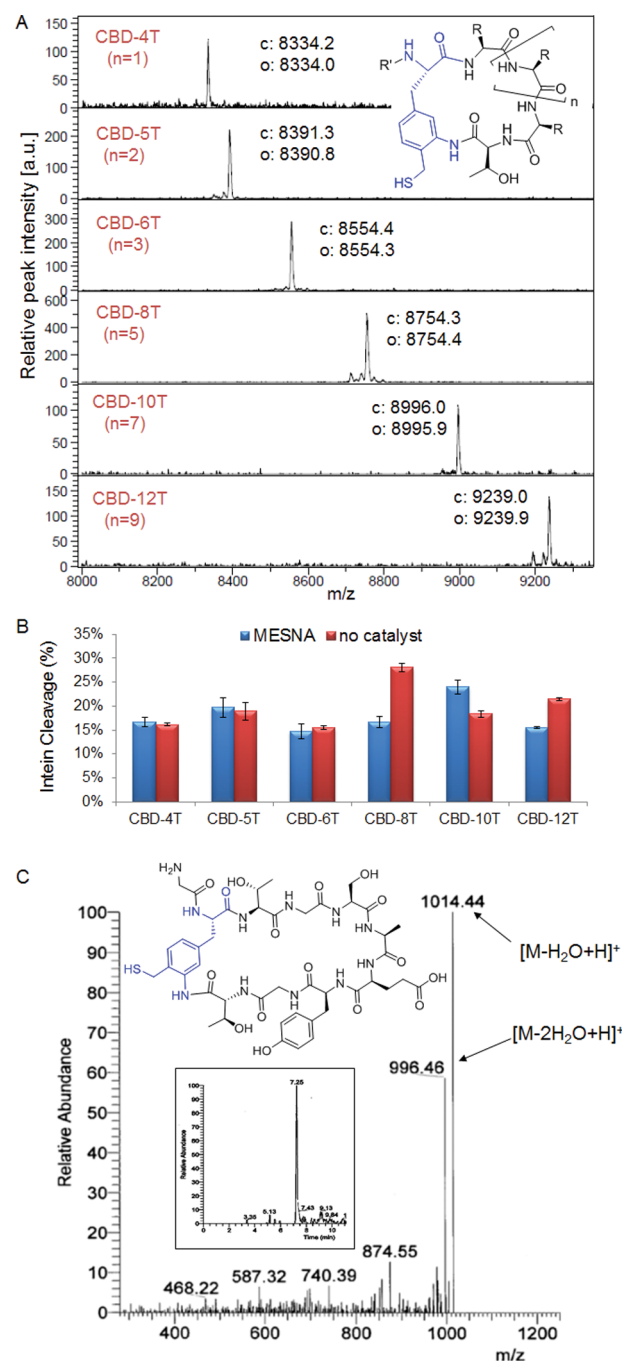
Figure 4. pH-induced cyclization of AmmF-containing constructs in vitro . (A) MALDI-TOF MS spectra of the macrocyclic peptides generated under catalyst-free conditions. The calculated (c) and observed (o) m/z values corresponding to the [M + H]^+ adduct of the macrocyclic product are indicated. R' = chitin binding domain. (B) Extent of intein cleavage for constructs CBD-4T(AmmF) through CBD-12T(AmmF) at pH 5.0 after 24 h as determined by SDS-PAGE. (C) Chemical structure, extracted-ion chromatogram (inset), and MS/MS spectrum of the macrocyclic peptide obtained from pH-induced cyclization of the MG-8T(AmmF) construct. Calculated m/z values for the [M - H_2O + H]^+ and [M - 2H_2O + H]^+ species are 1014.07 and 996.05, respectively.
