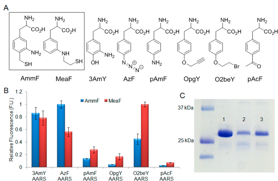
Figure 2. Orthogonal aminoacyl-tRNA synthetases for ribosomal incorporation of the aminothiol amino acids. (A) Structures of the target amino acids, AmmF and MeaF, and other UAAs mentioned in the text. (B) Relative fluorescence measured in the YFP reporter assay for the panel of AARSs in the presence of AmmF or MeaF. Data are normalized to the highest value within each series. (C) SDS-PAGE analysis of purified wild-type YFP (lane 1) and YFP variants incorporating AmmF (lane 2) and MeaF (lane 3).
