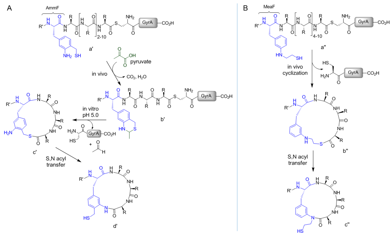
Figure 3. Precursor polypeptides, reaction intermediates, and final macrocyclic peptide products for (A) AmmF-mediated and (B) MeaF-mediated peptide cyclization. (A) Expression of the AmmF-containing precursor protein (a') in E. coli results in the formation of the benzothiazine adduct (b'), which, upon pH-induced deprotection in vitro , leads to the target macrocyclic peptide (d'). (B) Expression of the MeaF-containing precursor protein (a'') in E. coli results in spontaneous, post-translational peptide cyclization to give the thiolactone intermediate (b'') and then the final macrolactam product (c'') via an S → N acyl shift rearrangement.
