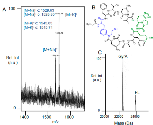
Figure 7. Isolation of streptavidin-binding peptide macrocycle from E. coli . (A) MALDI-TOF spectrum and (B) chemical structure of the cyclo (Strep1) as isolated from E. coli cells using streptavidin-coated beads. The HPQ motif is highlighted in green. (C) LC-MS spectrum of the Ni-affinity purified full-length precursor protein (FL) and spliced GyrA intein (GyrA) illustrating the extent of intein cleavage occurring in vivo .
